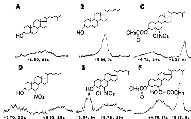
Fig. 1.—Determination of configuration in steroids by means of nuclear magnetic resonance. The first number below each peak is the chemical shift in \tau units. The second number is the width of the band at half-height ( W^{1/2} ) in c.p.s., and the letter a (axial) or e (equatorial) denotes the configuration of the proton responsible for the band. There are two errors in this figure: A should read \tau 6.50, 25a; E should read \tau 5.34, 6e, and \tau 5.78, 23a.
